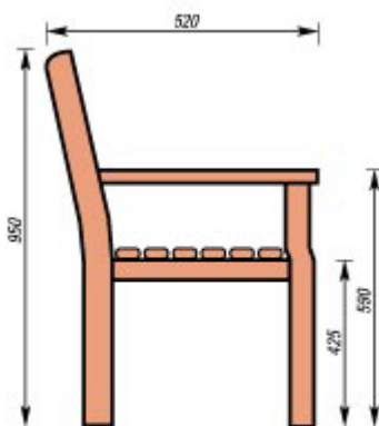
TRADITIONAL SEAT WITH FLAT ARMS
