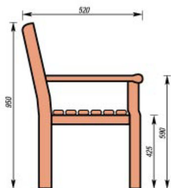
NEW TRADITIONAL SEAT WITH ROLL ARMS
